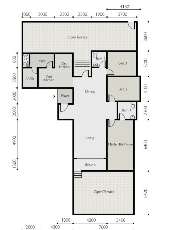
TYPE F Built-Up - 145 sq.m. (1561 sq.ft.) Open Terrace - 102 sq.m. (1098 sq.ft.)
