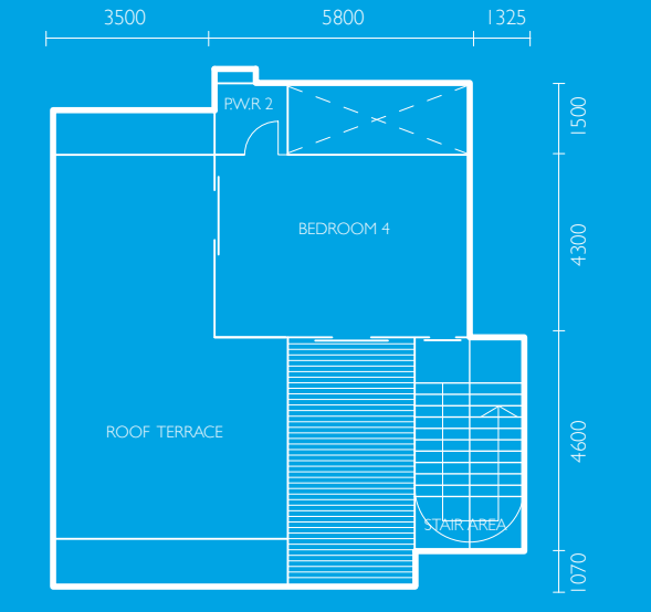
Type E/E1 - Level 3
