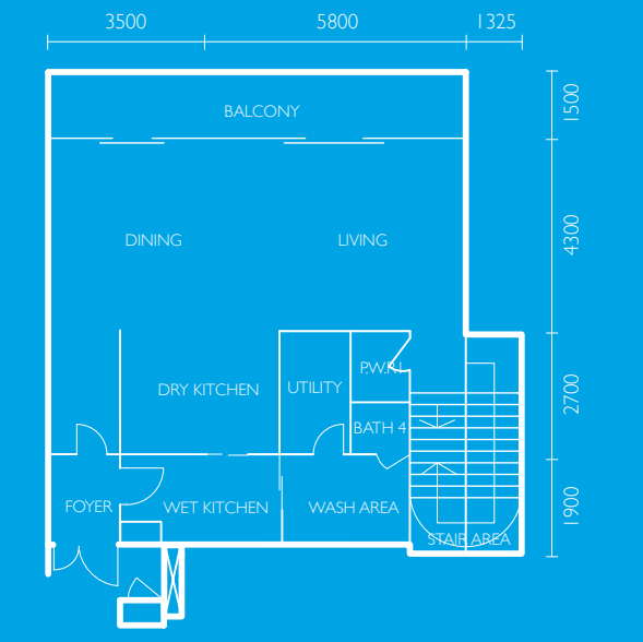
Type E/E1 - Level 1
