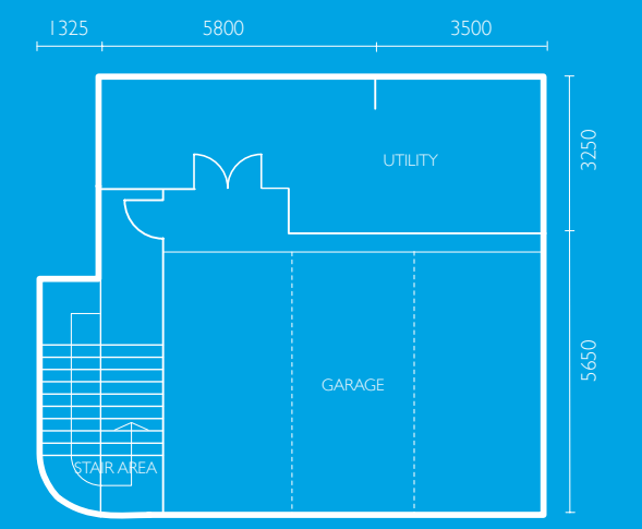
Type E1 - Basement - 290m 2 (3122sf) - Main Parcel, 111m 2 (1195sf) - Accessory Parcel
