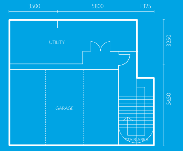
Type E - Basement - 291m 2 (3132sf) - Main Parcel, 111m 2 (1195sf) - Accessory Parcel
